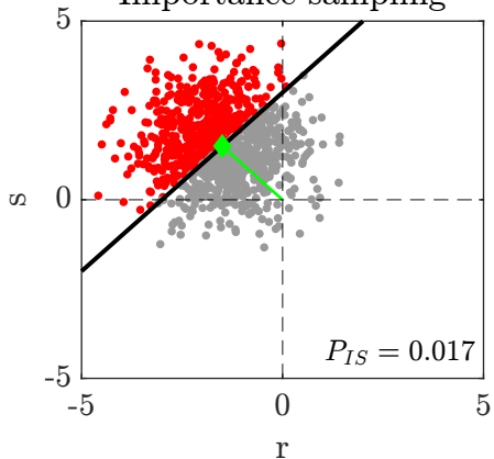
Importance sampling
